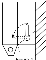
Figure 4 Keeping the clapper closed while the system is in operation will ensure maximum heat efficiency.
