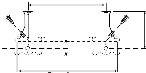
Figure 3 a Distance between the bracket slide ends (mm) = (80x Number of Radiator Columns) – 5mm
